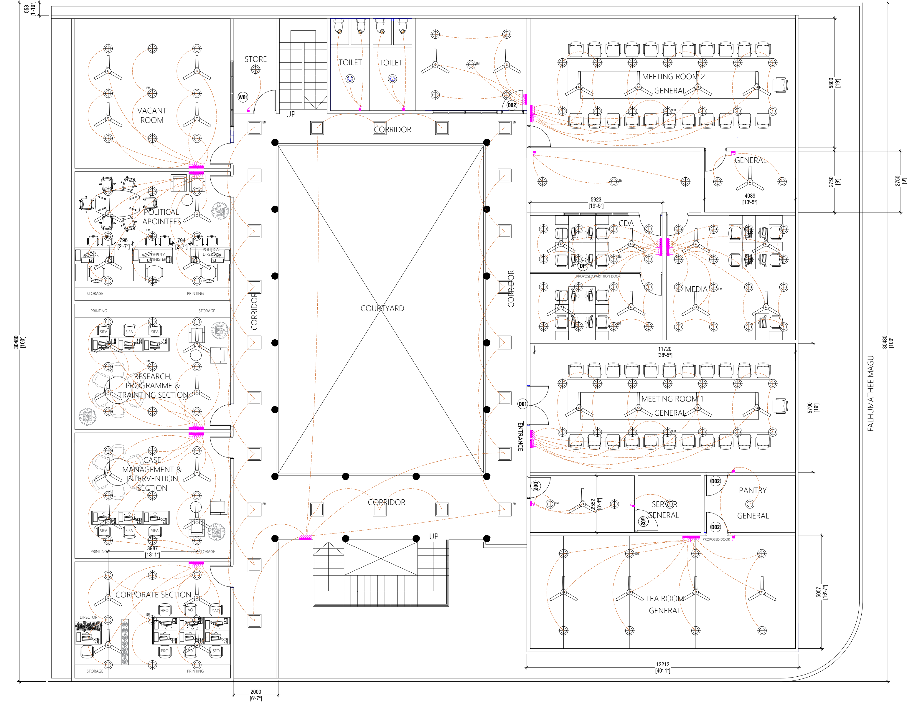
THIRD FLOOR EXISTING FLOOR PLAN (LIGHTING LAYOUT)
