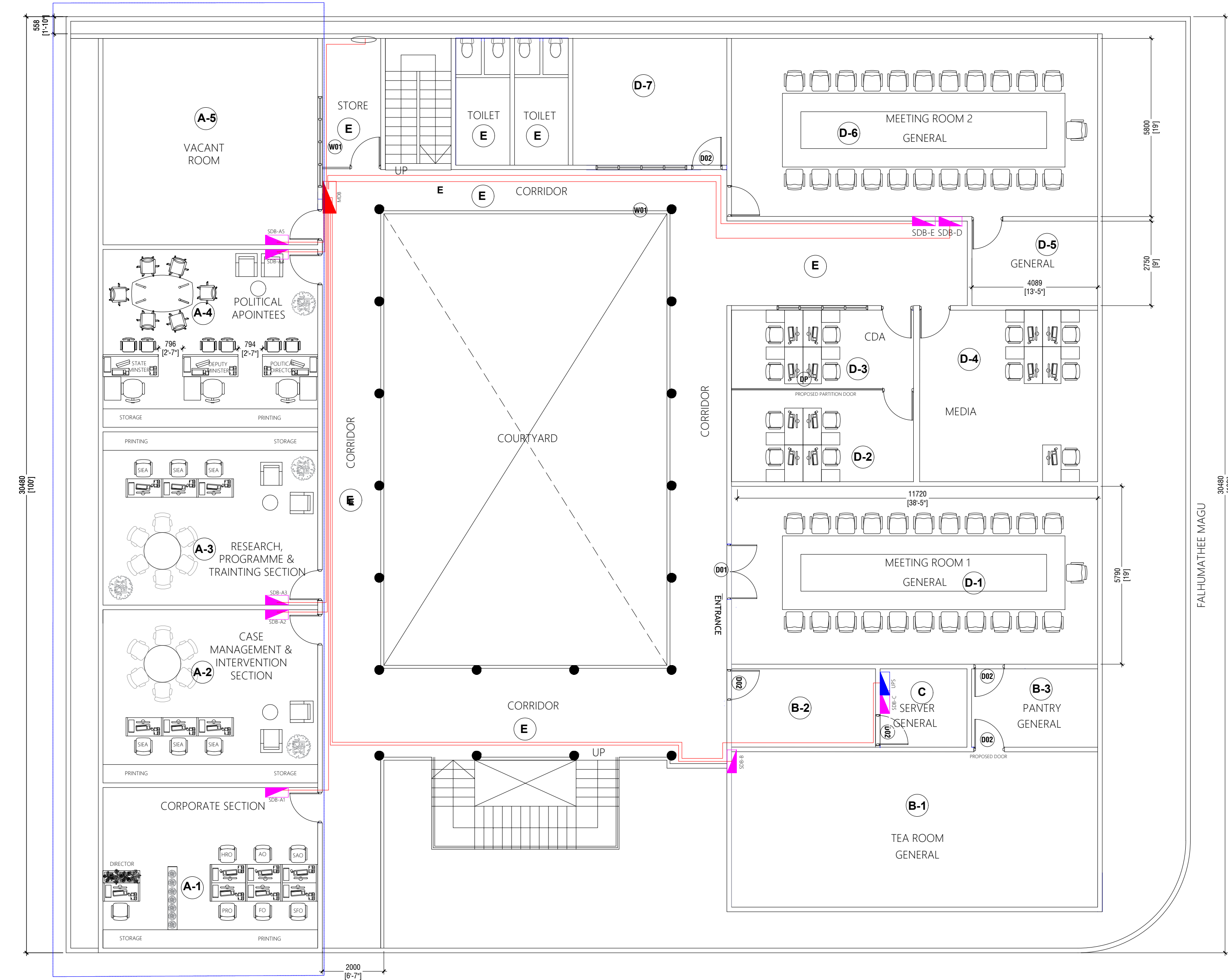
THIRD FLOOR EXISTING FLOOR PLAN (POWER DISTRIBUTION LAYOUT)
