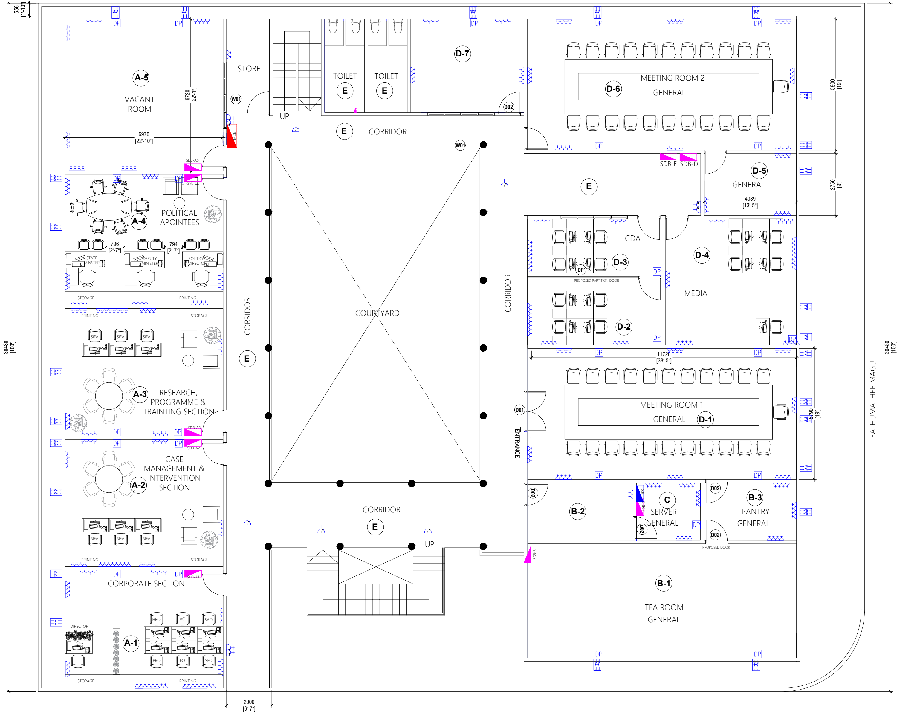
THIRD FLOOR EXISTING FLOOR PLAN (POWER LAYOUT)
